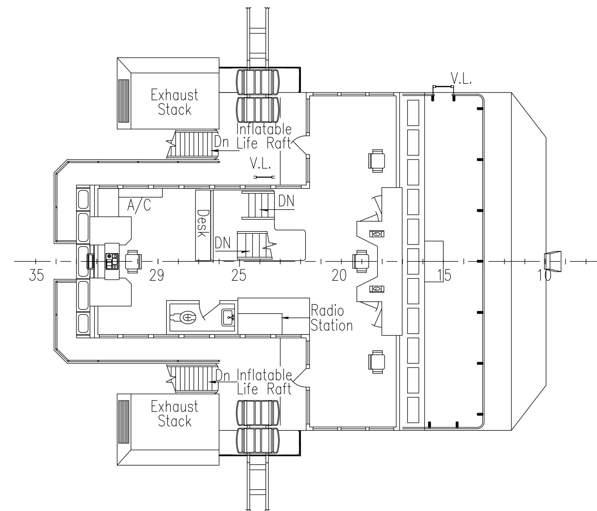
BRIDGE DK LEVEL 41'-10" ABOVE BASELINE
